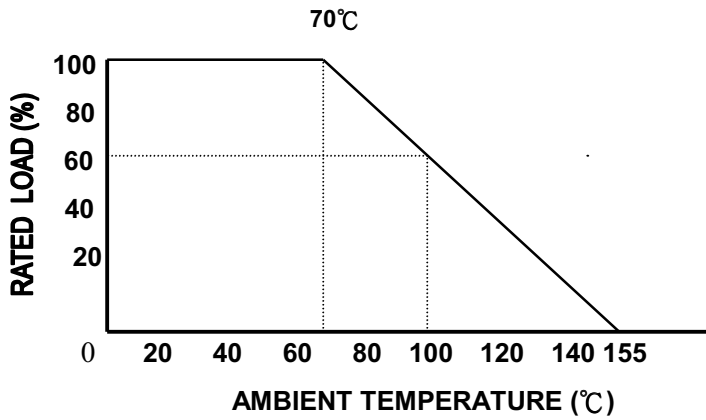
FIG.1 DERATING CURVE
