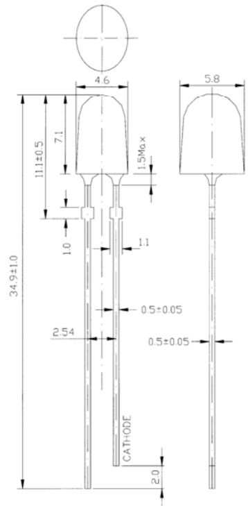
Dimensions (Unit: mm)
