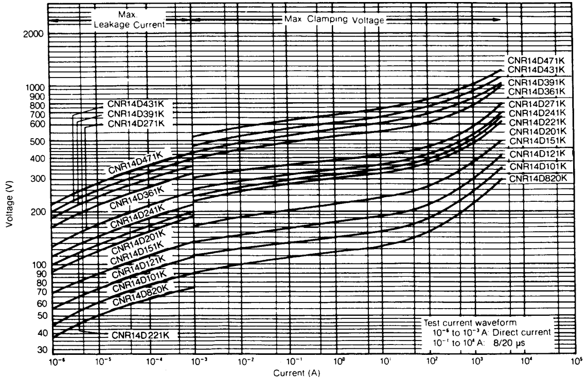
V-I Curve (CNR14D820K to CNR14D471K)
