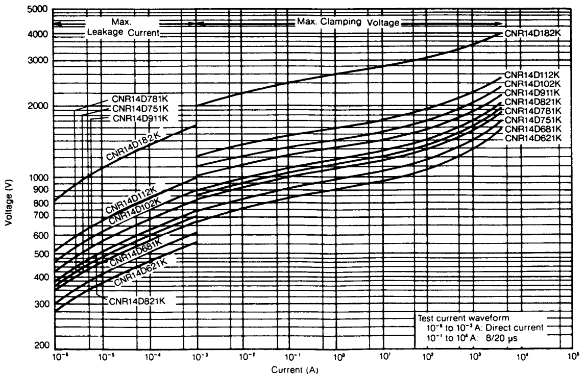
V-I Curve (CNR14D621K to CNR14D182K)
